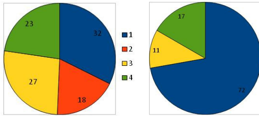
Figure 4: percentage of application of each of the parameters in the European (left) and American (right) surveys. 1: Destructive Potential; 2: Runout classification; 3: Typical length; 4: Typical mass/volume.
