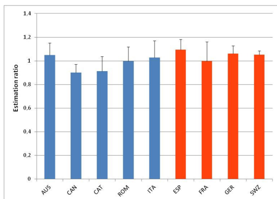
Figure 5: Estimation Ratio per country. This ratio comes from dividing every classification in the survey by the average of the classifications for this case. In blue, countries with 9 or more surveys, in orange countries with 2 to 4 cases.
