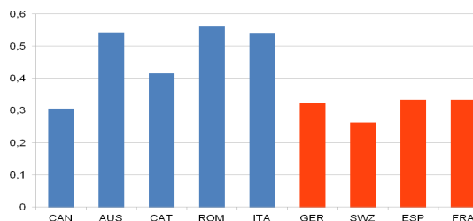
Figure 3: Standard deviation values plotted by country. In blue, the countries with 9 or more surveys, in orange countries with 2 to 4 surveys.
